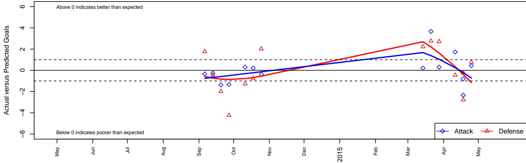
BC United Diablitos B01 Dots are actual minus expected GF (blue circles) and GA (red triangles). Blue line is smoothed change in attack strength. Red is smoothed change in defense strength.
